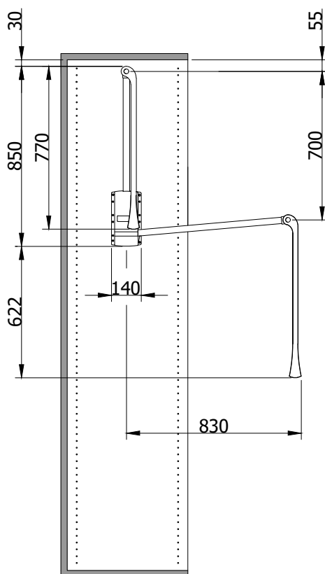
BIANCO - CROMATO white - chrome-plated
