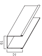
Guida in ferro GUFERSM 19 x 22 mm
