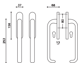
L102
