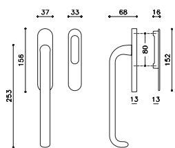
L101
