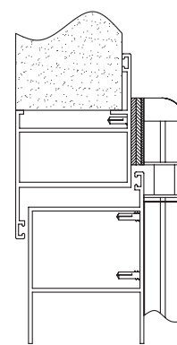
Apertura interna con sormonto Internal overlapped opening
