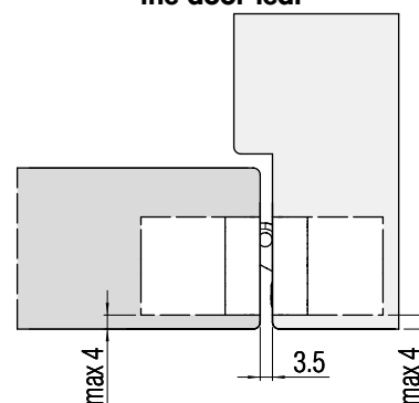
Installation of the door leaf
