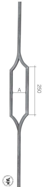
Art. GD25/3 \varnothing 14 mm 110 x 1000 mm A = 82 mm Art. GD243/2 \varnothing 12 mm 110 x 1000 mm A = 86 mm
