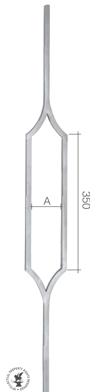
Art. GD25/2 \varnothing 14 mm 110 x 1000 mm A = 82 mm Art. GD243/1 \varnothing 12 mm 110 x 1000 mm A = 86 mm
