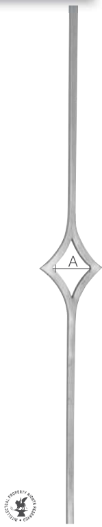
Art. GD23/1 \varnothing 14 mm 120 x 1000 mm A = 75 mm Art. GD58/3 \varnothing 12 mm 120 x 1000 mm A = 80 mm
