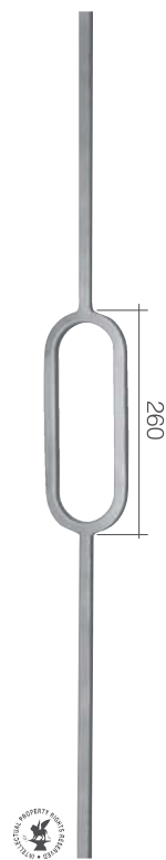
Art. GD29/1 \Phi 14 mm L 100 mm H 1000 mm
