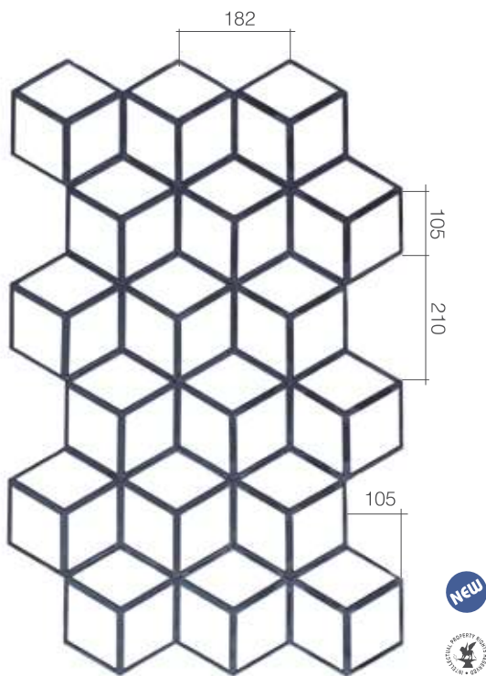
Art. GD287/4 \square 12 x 6 mm + \Phi 12 mm H 1000 mm L 638 mm
