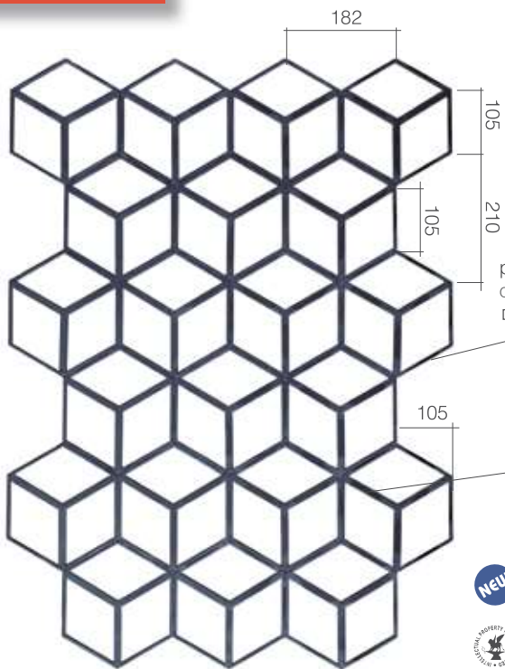
Art. GD287/1 \square 12 x 6 mm + \Phi 12 mm H 1000 mm L 728 mm
