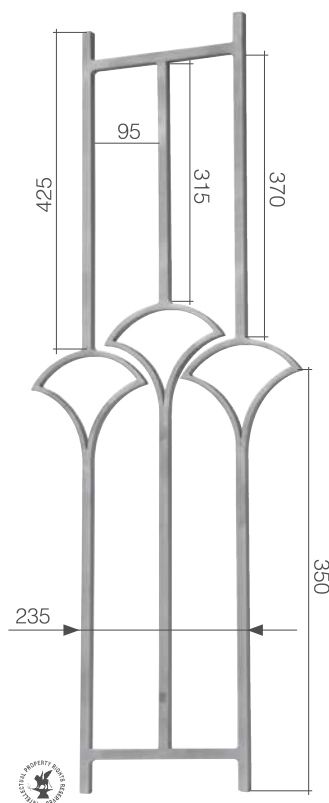
Art. GD186/3 \varnothing 14 mm L 390 mm H 1000 mm
