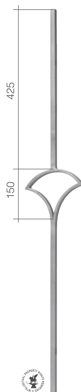
Art. GD186/1 \varnothing 14 mm L 170 mm H 1000 mm
