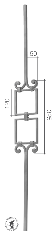
Art. GD184/1 \Phi 14 mm L 115 mm H 1000 mm
