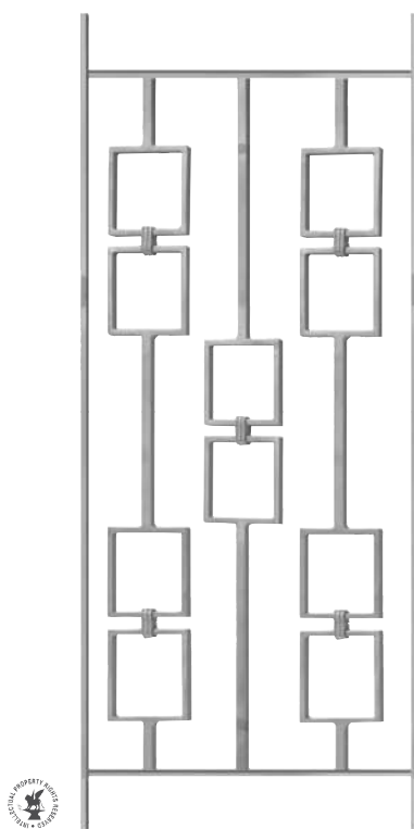
Art. GD183/1 \square 14 x 8 mm L 400 mm H 1000 mm
