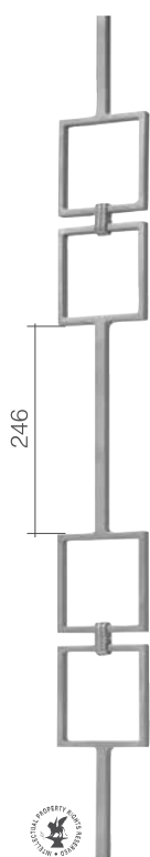
Art. GD182/2 \Phi 14 mm L 115 mm H 1000 mm
