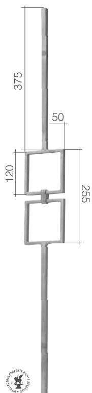
Art. GD182/1 \Phi 14 mm L 115 mm H 1000 mm
