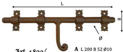
Art. 1890/ Catenaccio Bolt
