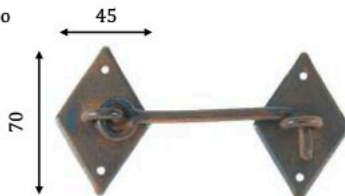
Art. 2132/ Chiavistello/Cabin hook A 145mm- Asta/Hook 100mm B 195mm- Asta/Hook 150mm
