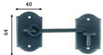
Art. 2133/ Chiavistello/Cabin hook A 145mm- Asta/Hook 100mm B 195mm- Asta/Hook 150mm
