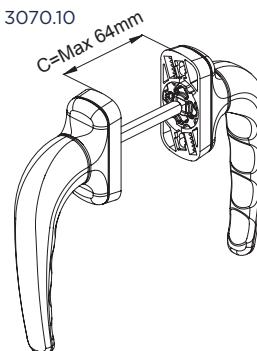
Art. 3070.10
