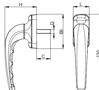
Art. 3070.10
