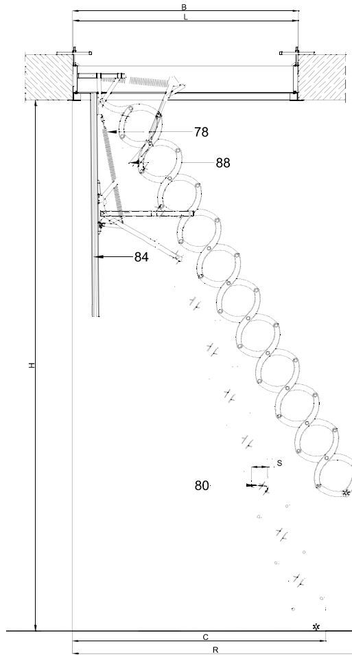
78-Spring 80-Tread 84-Thermo-insulated hatch 88-Side bracket
