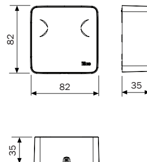
Cable Free RFID - LED only (art. 5E1511155)
