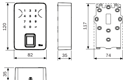
Cable Free RFID with keyboard and fingerprint (art. 5E1511355)
